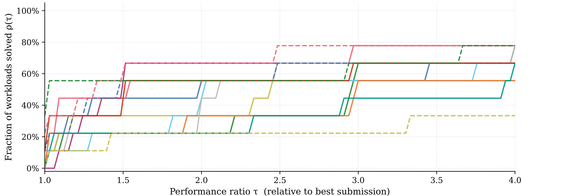
AlgoPerf: Self-Tuning Ruleset Performance Profiles (targets relaxed 10%)
