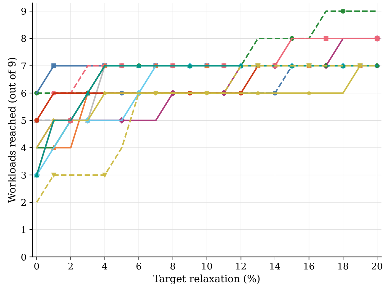
(b) Workloads reaching the target
