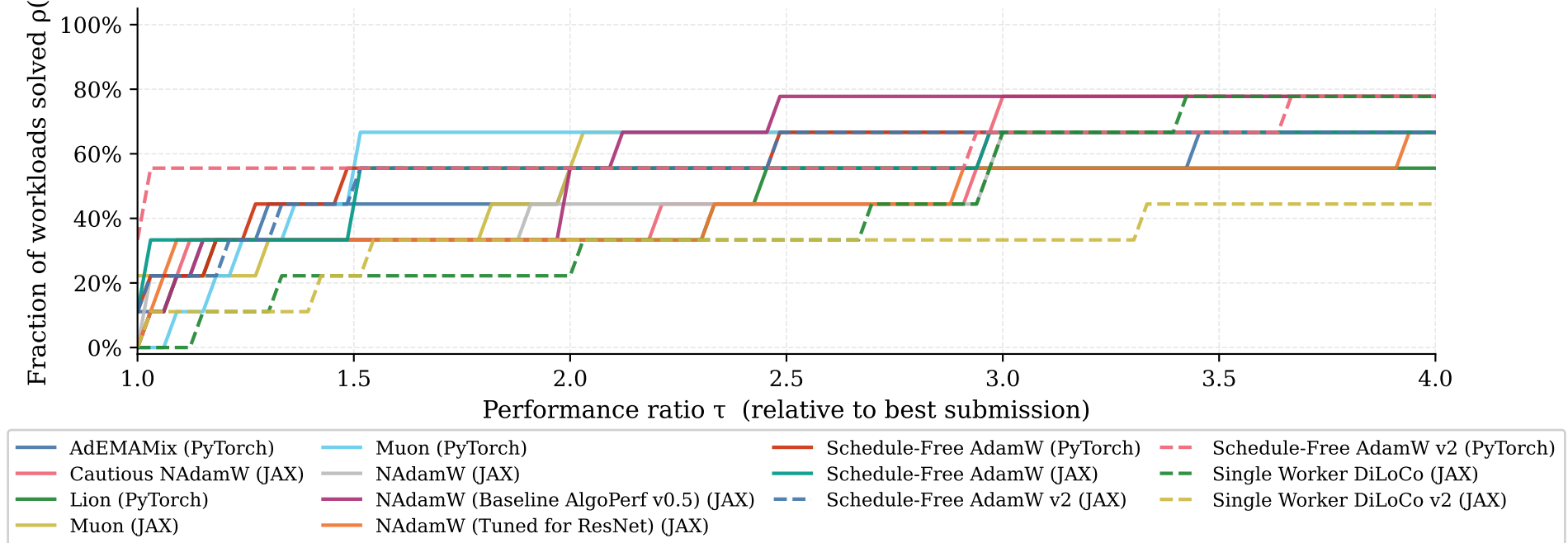
AlgoPerf: Self-Tuning Ruleset Performance Profiles (targets relaxed 10%)
