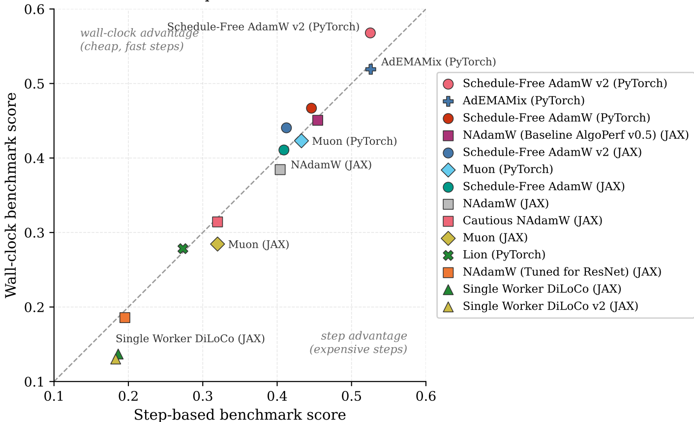
Wall-clock vs. step-based benchmark scores
