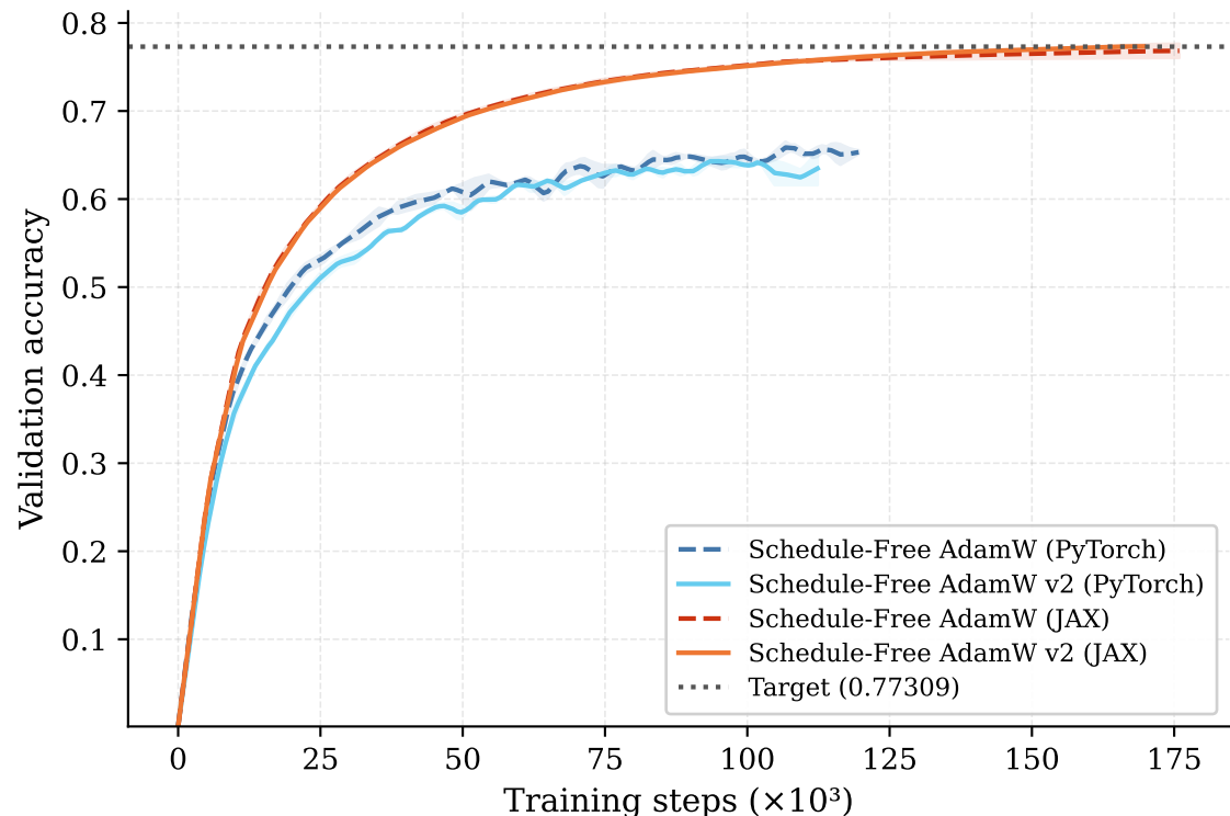
ImageNet ViT: validation accuracy
