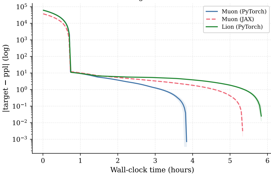
Distance to target vs. wall-clock time
