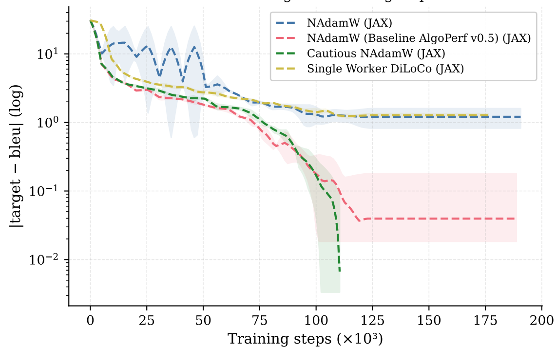
Distance to target vs. training steps
