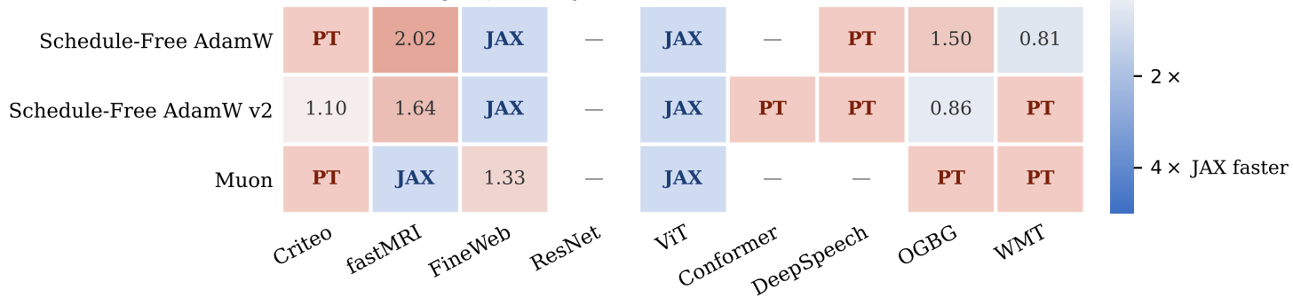
(b) Time to target, JAX \div PyTorch
