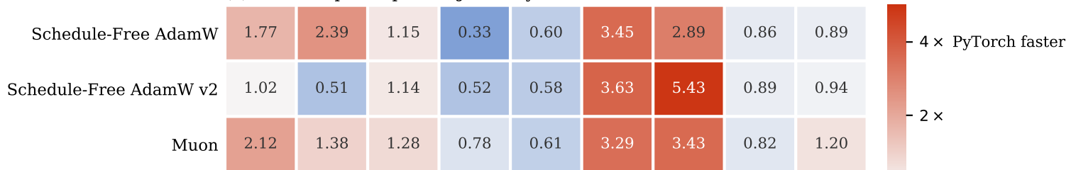
(b) Time to target, JAX \div PyTorch
