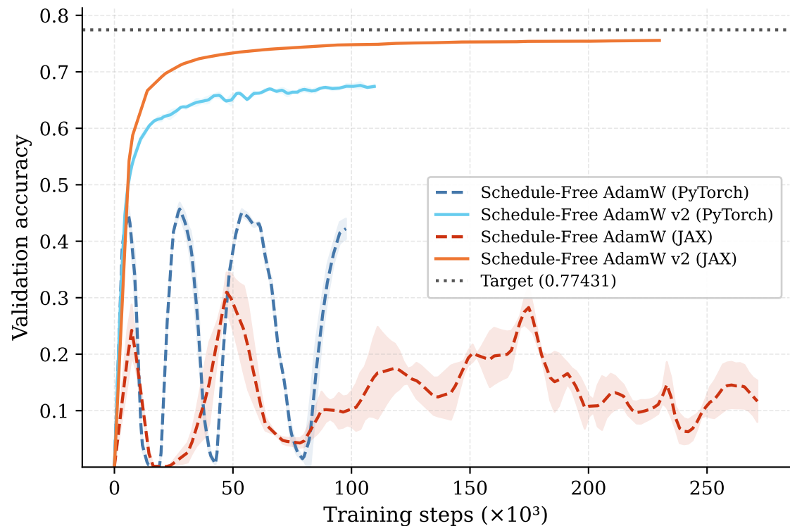
ImageNet ResNet-50: validation accuracy
