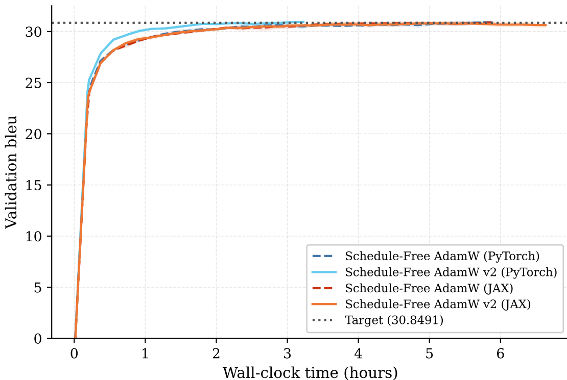
WMT Transformer: validation bleu
