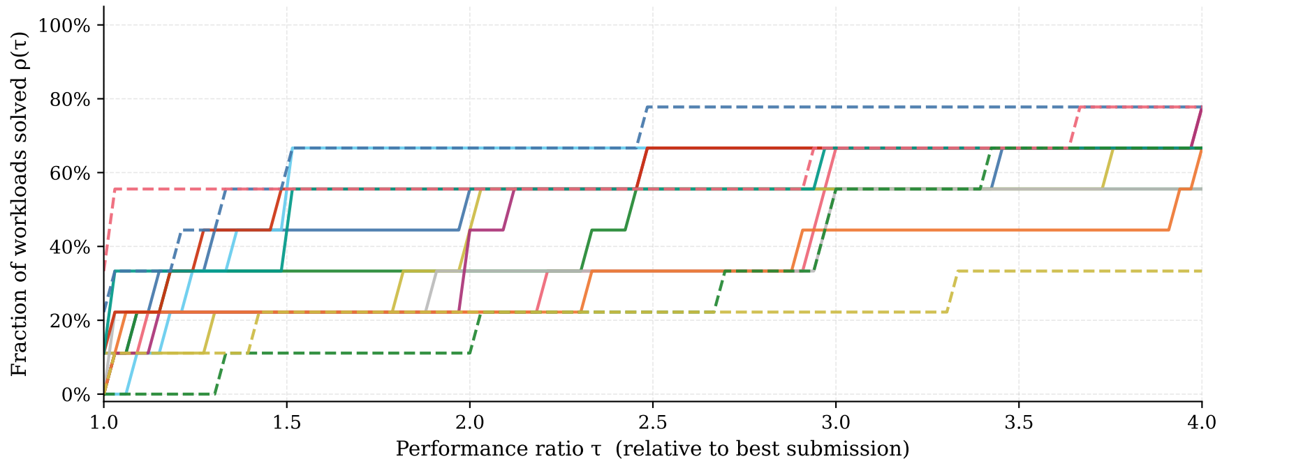
AlgoPerf: Self-Tuning Ruleset Performance Profiles (targets relaxed 10%)
