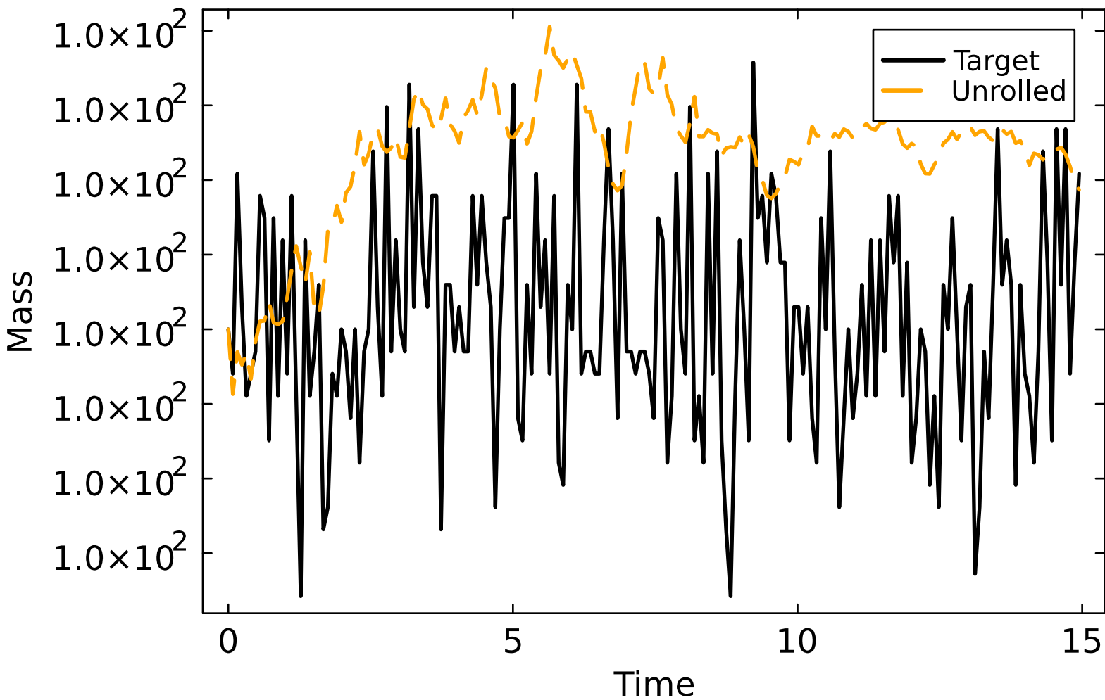
Mass conservation for Flux model
