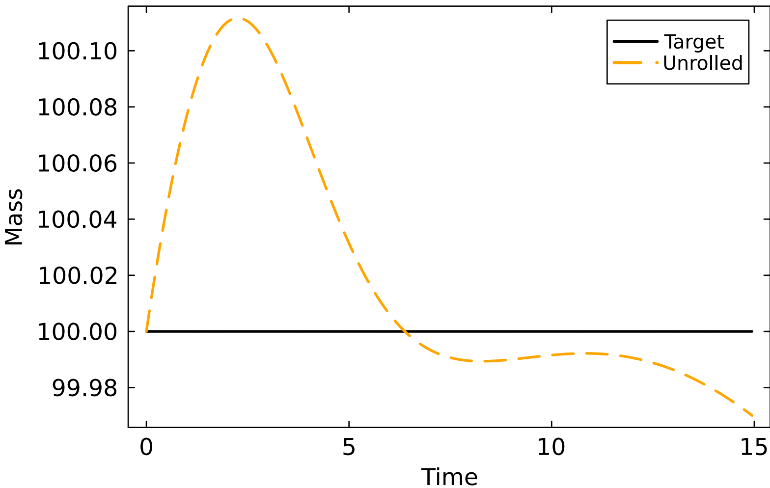
Mass conservation for standard CNN model
