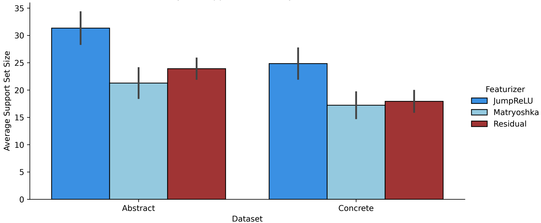
Feature Basis Analysis: Support Set Size by Dataset and Featurizer
