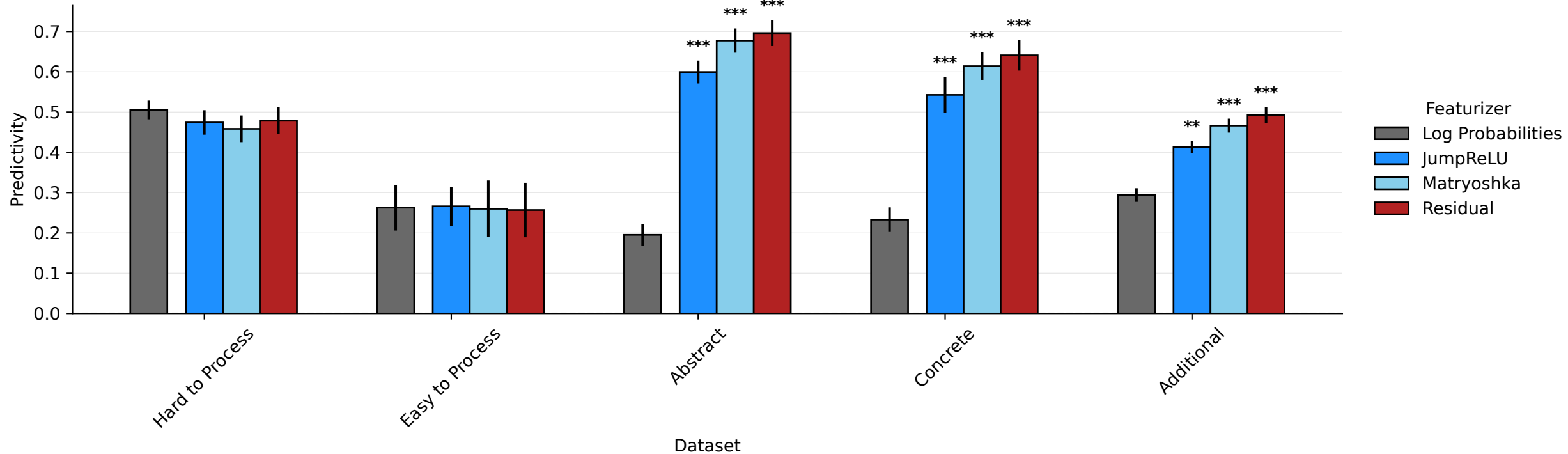
Predictivity by Dataset and Featurizer (Layer 14 Replication)
