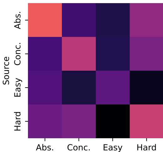
JumpReLU SAE Feature Generalization
