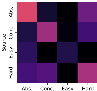
JumpReLU SAE Feature Generalization
