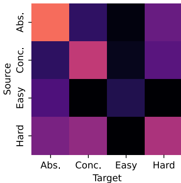
Residual Stream Feature Generalization
