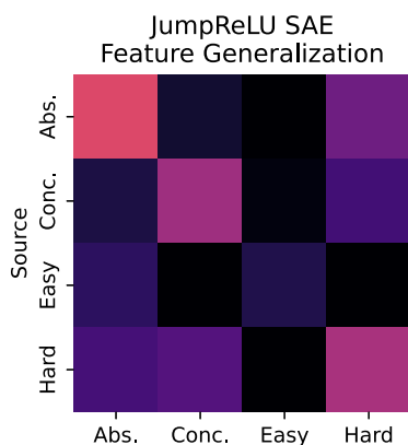
Generalization Between Abstract and Concrete
