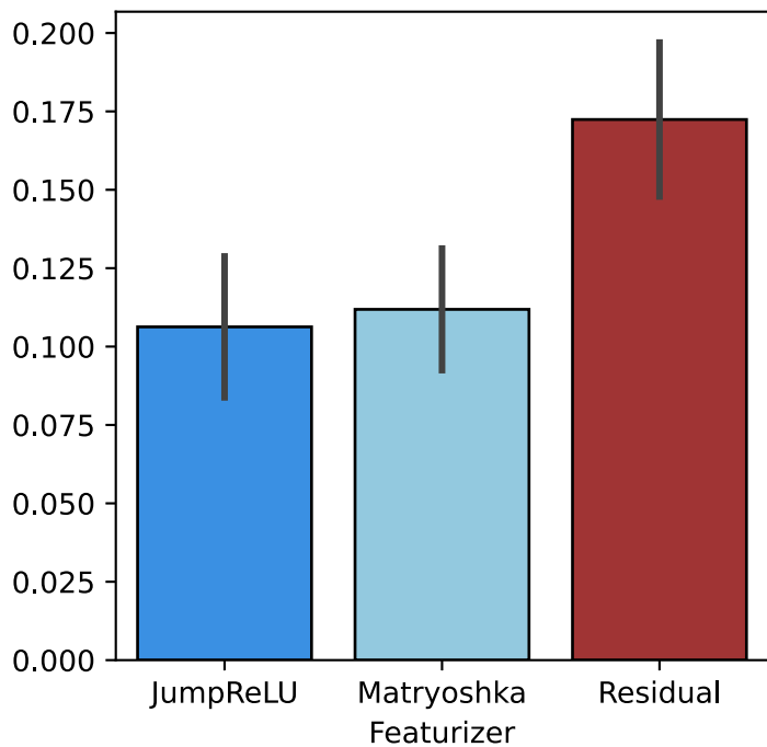
Generalization Between Abstract and Concrete
