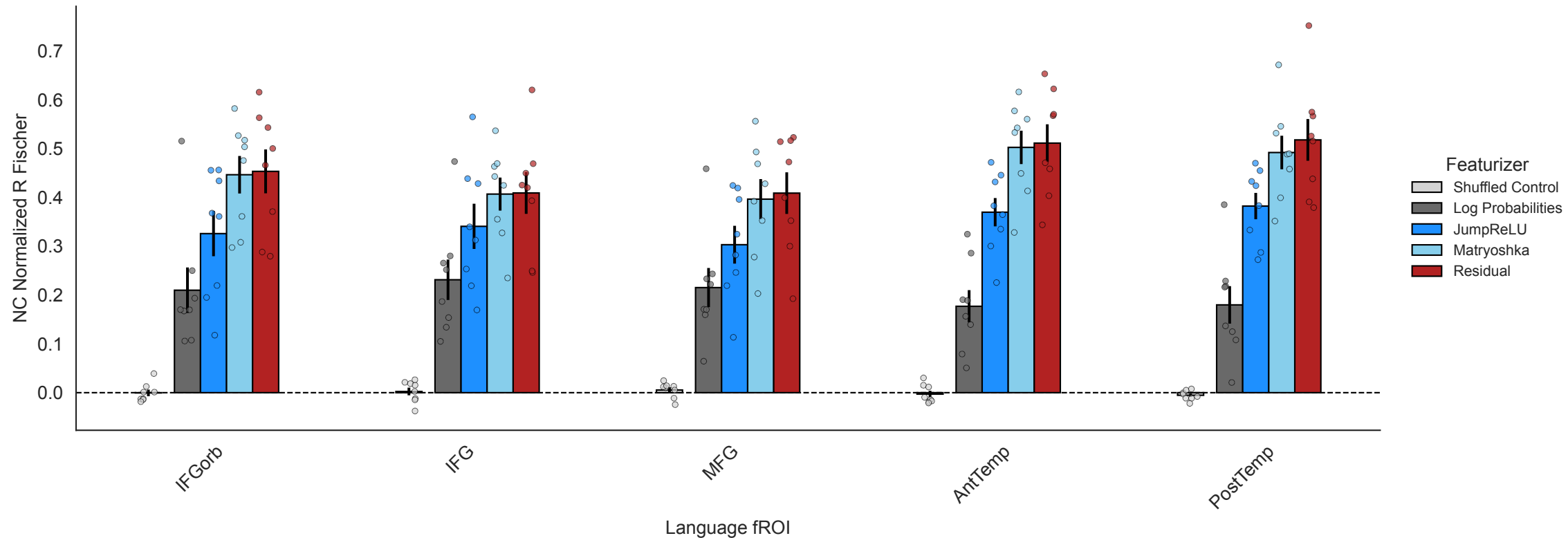
All voxels: NC Normalized R Fischer
