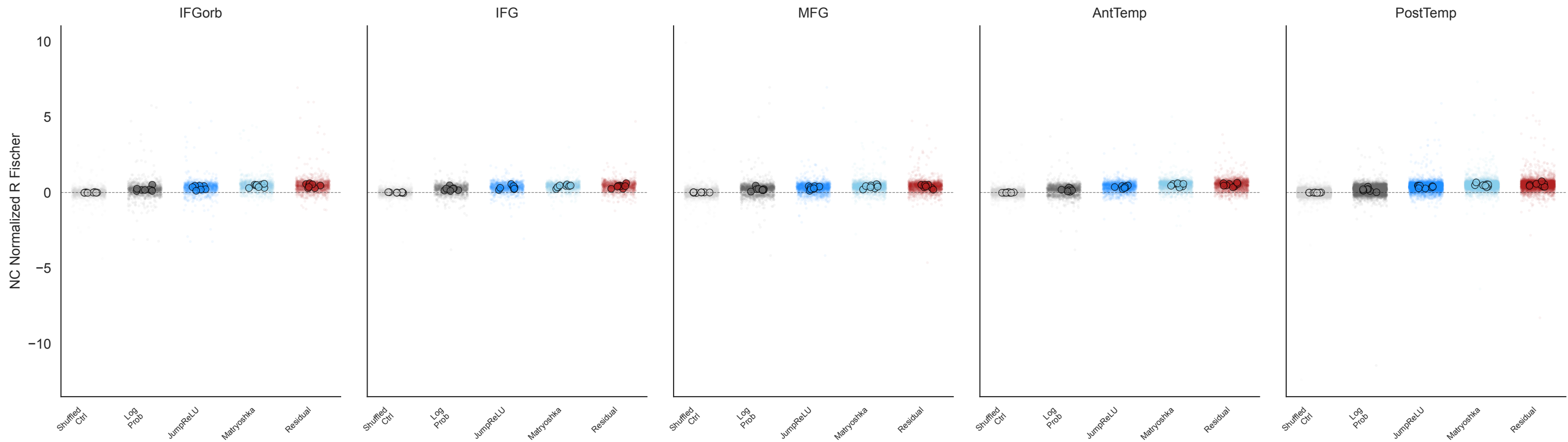
All voxels: NC Normalized R Fischer — voxel-level
