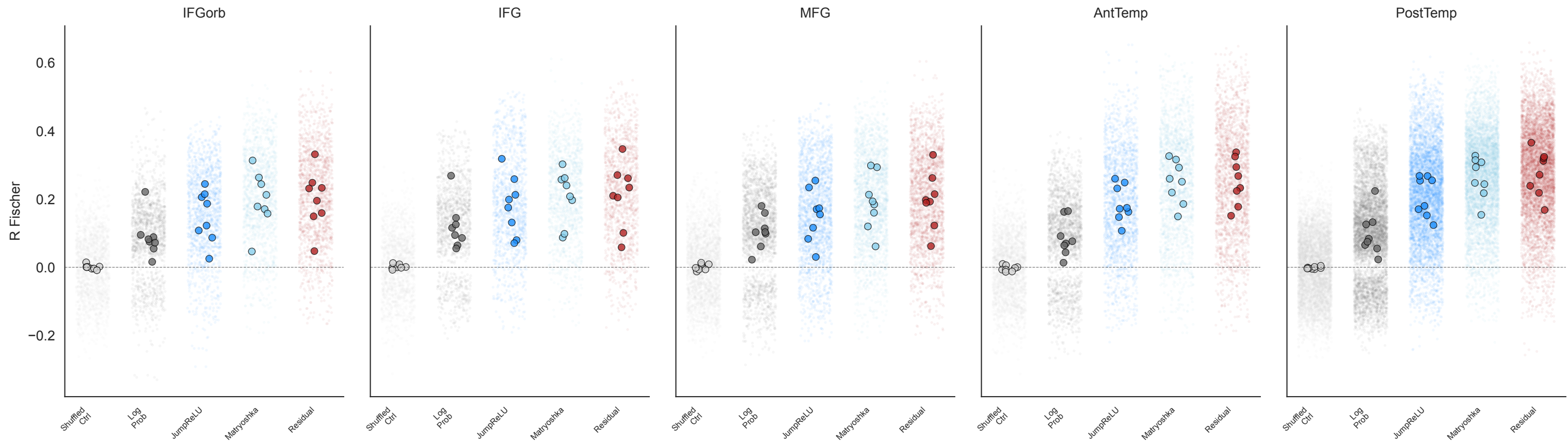
All voxels: R Fischer — voxel-level
