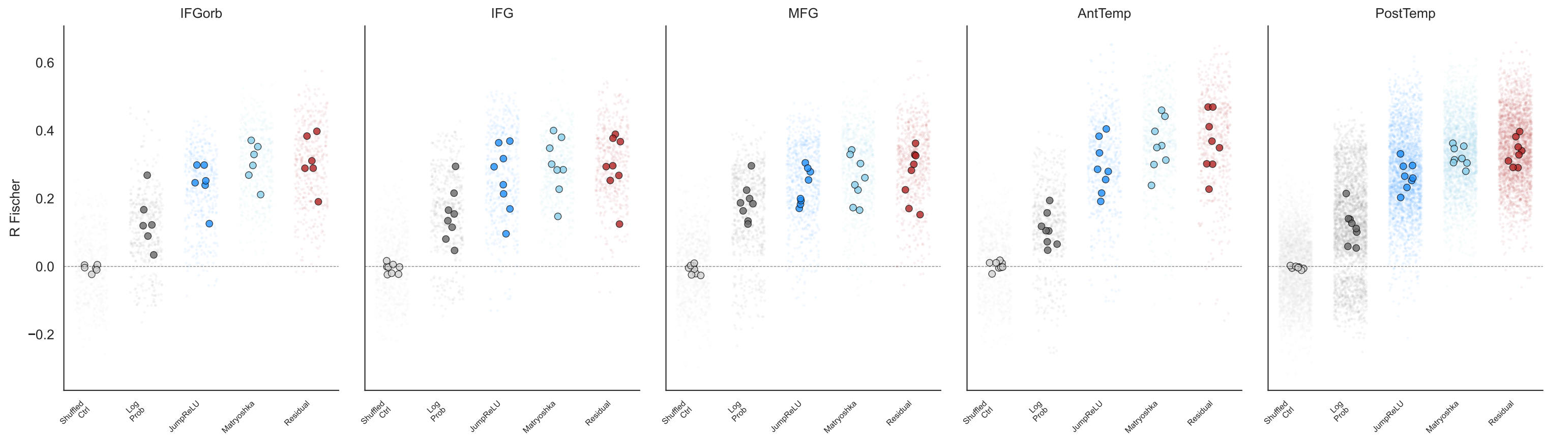
Filtered (NCSNR > 0.4): R Fischer — voxel-level
