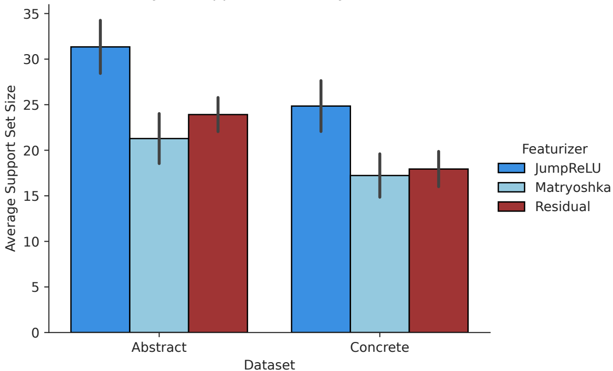
Feature Basis Analysis: Support Set Size by Dataset and Featurizer
