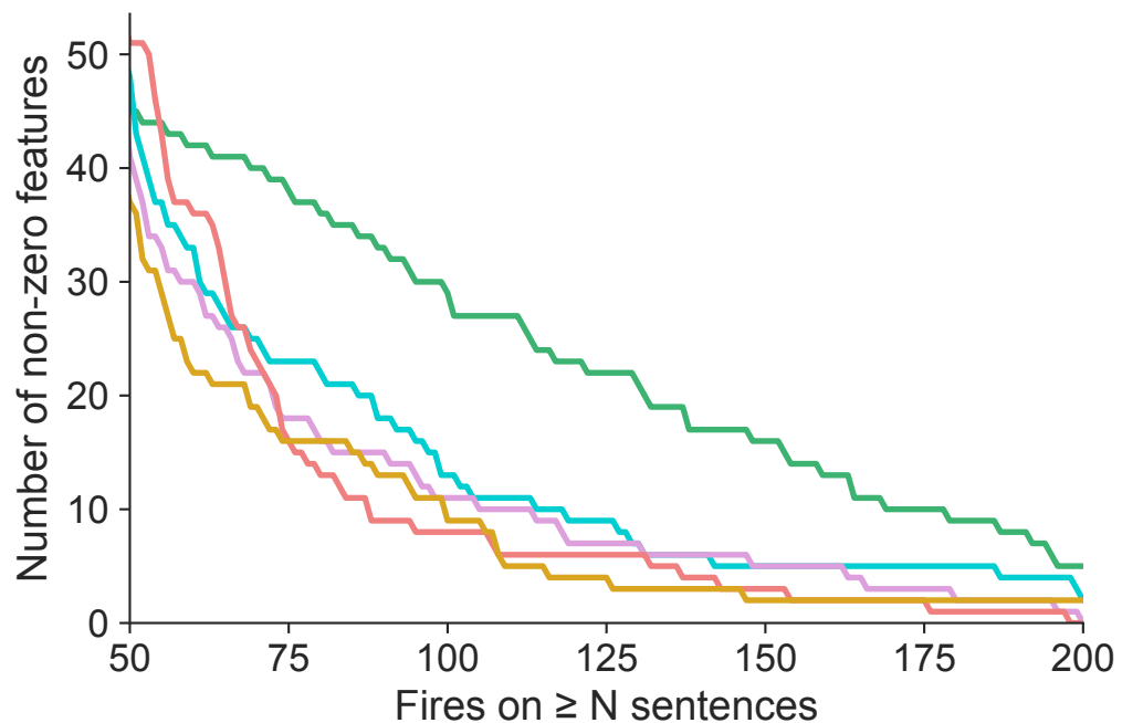
Zoom: 50–200 sentences
