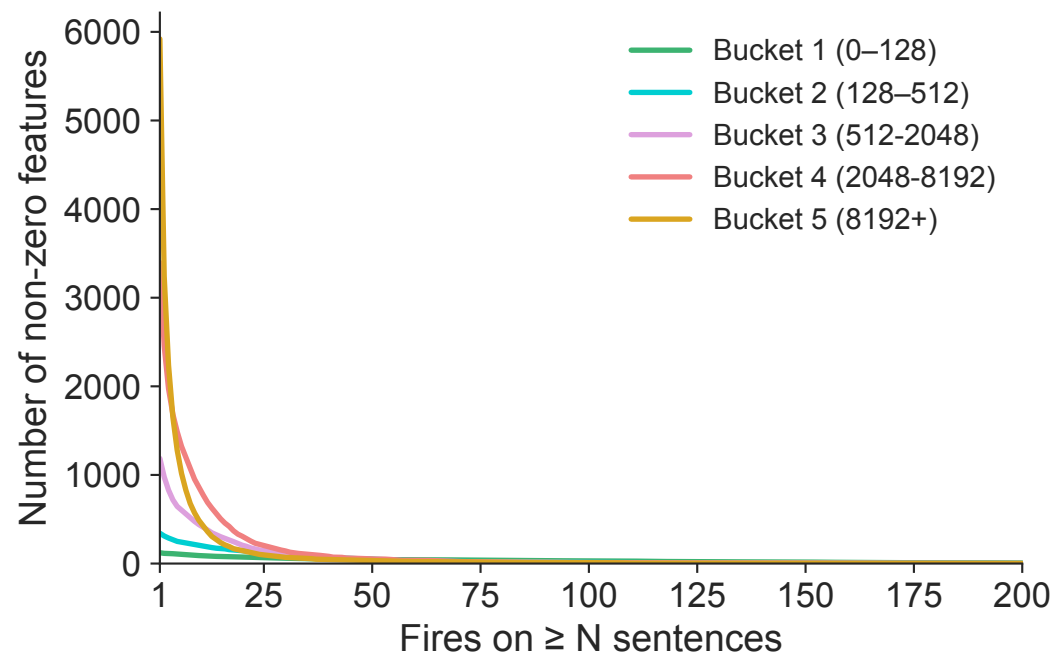
All sentences
