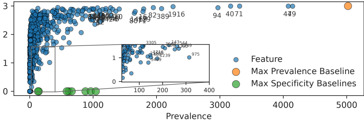
Entropy across Participants
