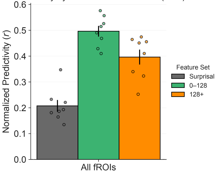
Predictivity by Restricted Feature Set (fROI)
