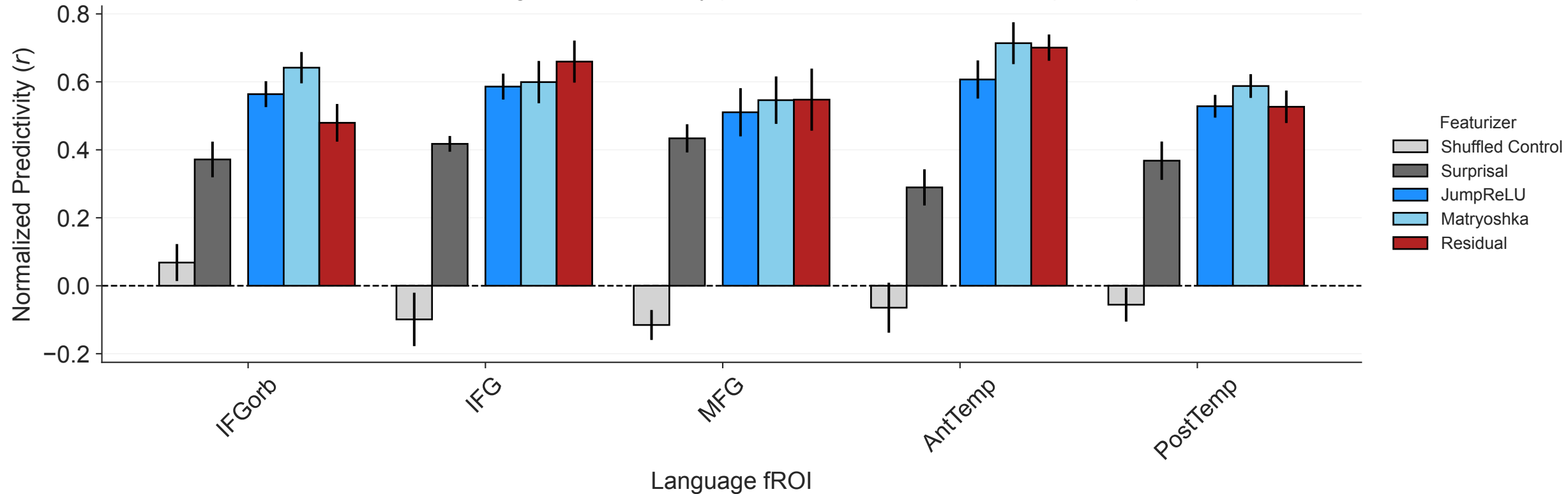
S3T Baseline Average: fROI Predictivity (corrected NC normalization, CV split SEM)
