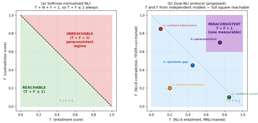
The Softmax Trap: why current hallucination detectors structurally cannot measure paraconsistency
