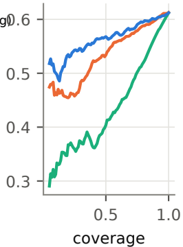
NQ-open
