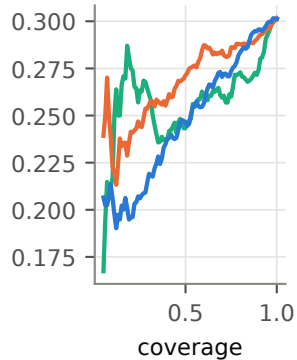
ChaosNLI
