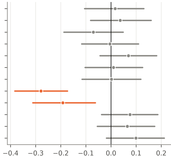
partial rank corr. of I with human entropy | scalar
