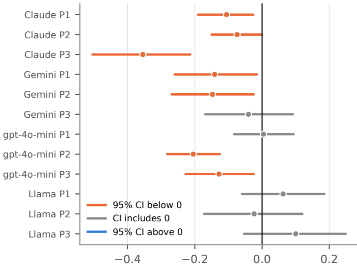
\rho(I, \text{human entropy}) - \rho(1\text{-scalar}, \text{human entropy})
