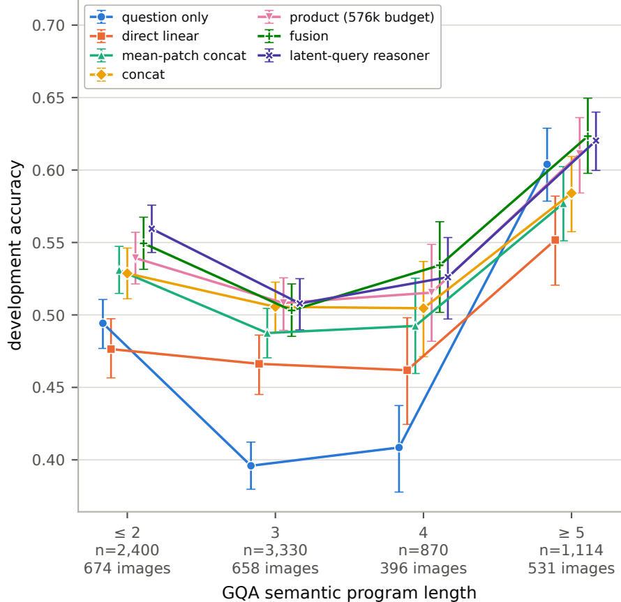
(a) accuracy by program length, train_40k — all seven systems
