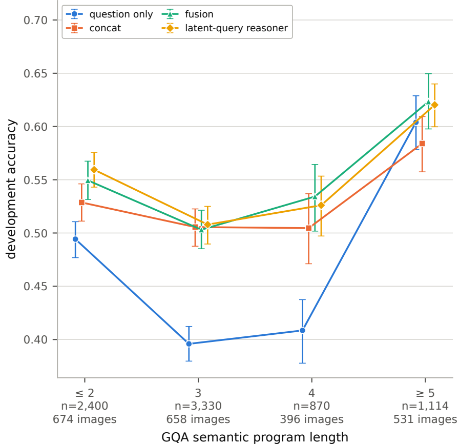
(a) accuracy by program length, train_40k — claim-driving systems
