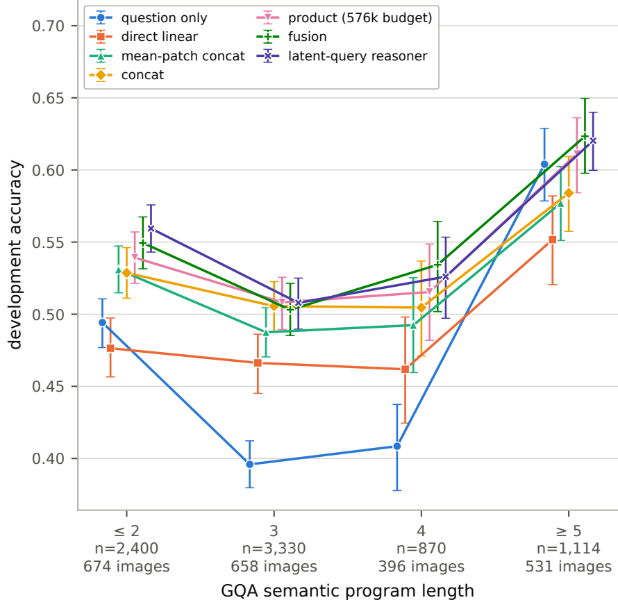
(a) accuracy by program length, train_40k
