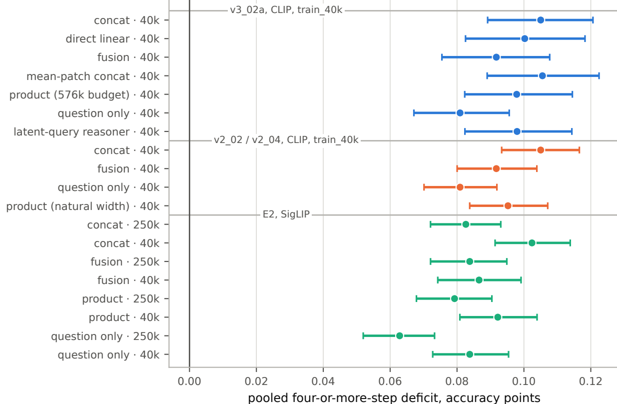
(b) pooled deficit against fixed v2_05b per-bucket priors
