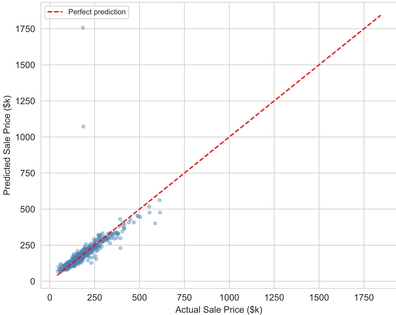
Figure 10 — FA-Only Regression: Actual vs Predicted R^2 = 0.814 | MAPE = 12.3% | 7 latent factors only
