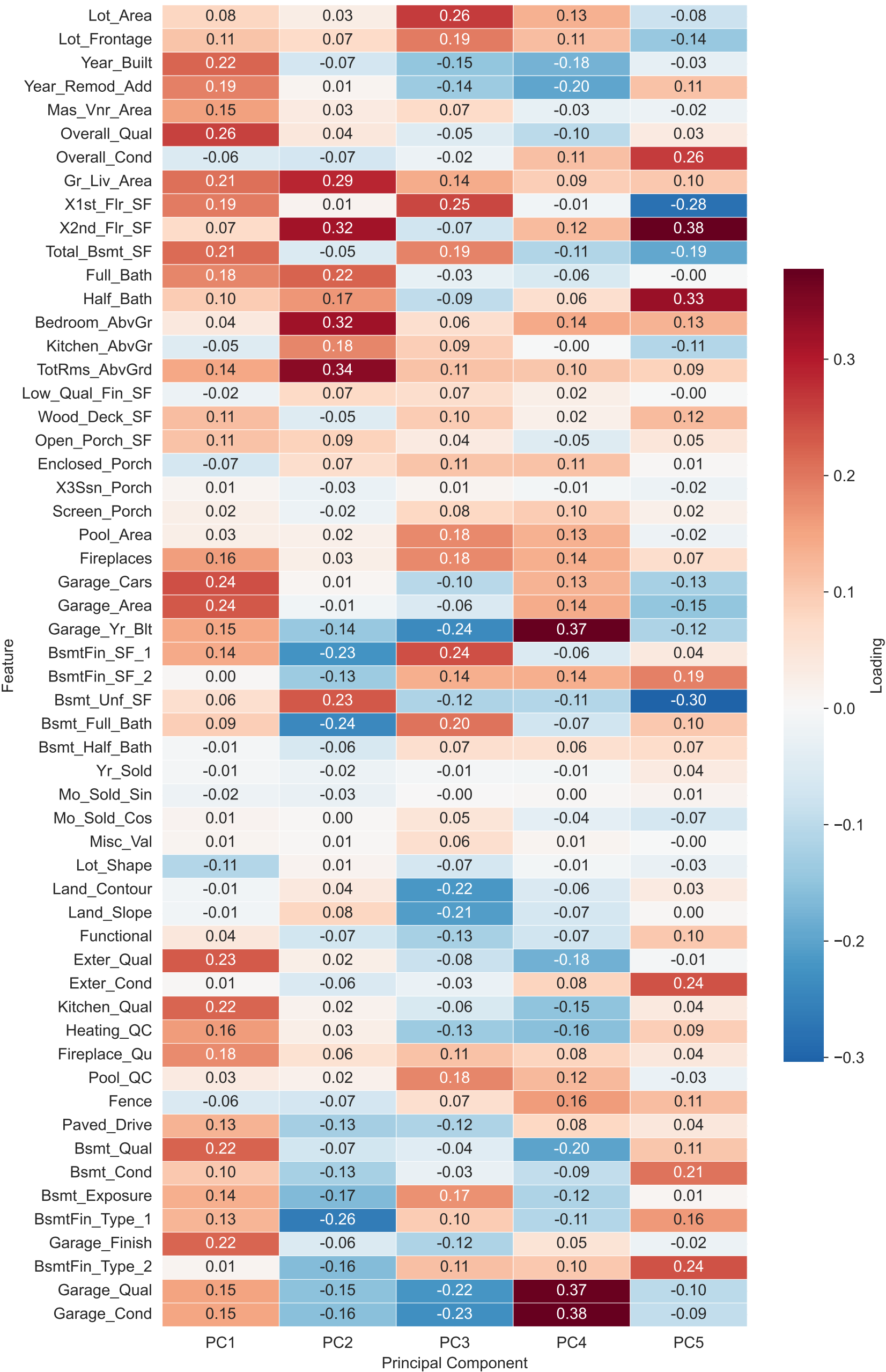
Figure 2 — PCA Loadings: First 5 Principal Components (red = positive, blue = negative)
