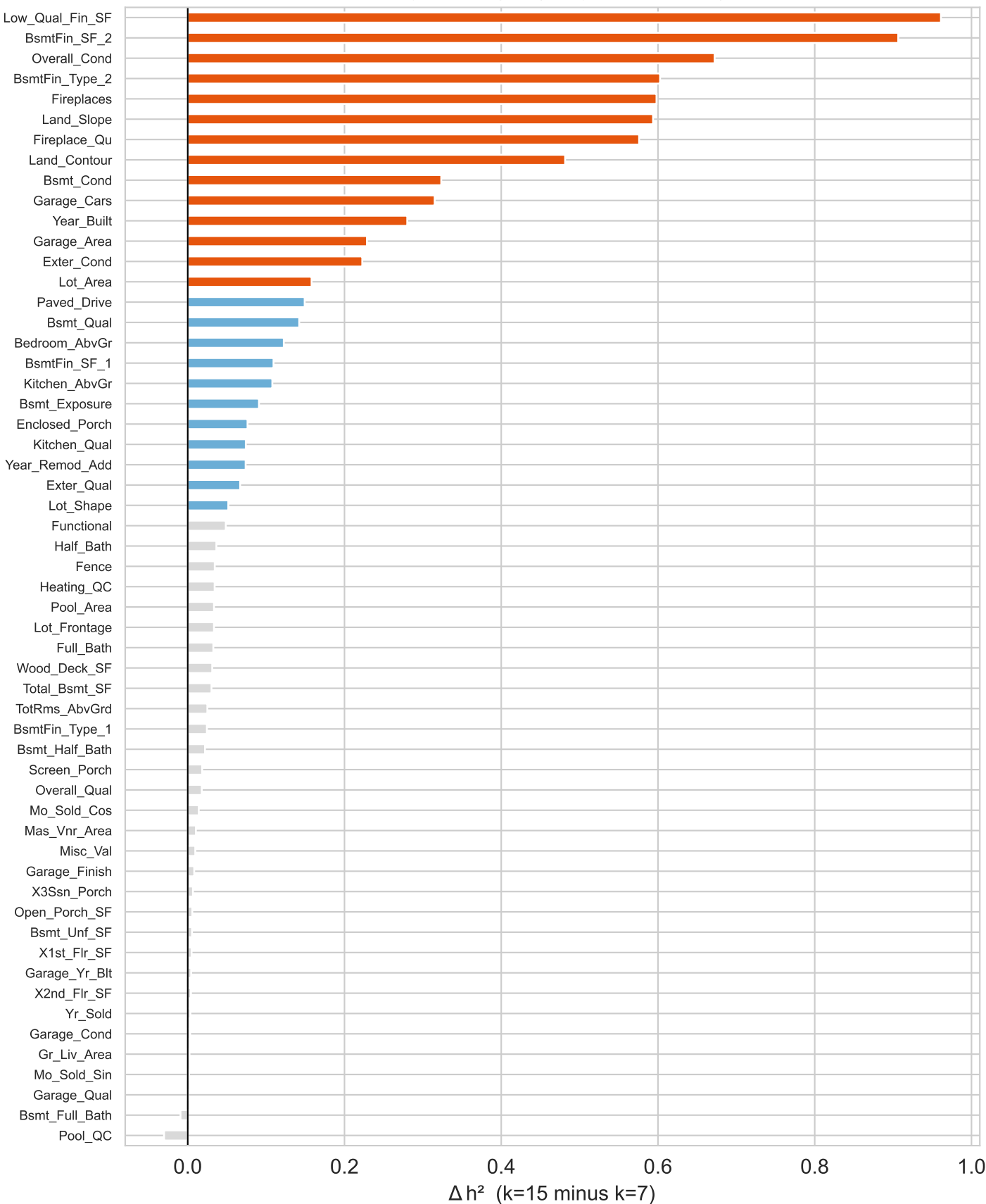
(b) Commuality Gain per Feature Orange: large gain (likely captured by new useful factors) Gray: little/no gain (idiosyncratic features)
