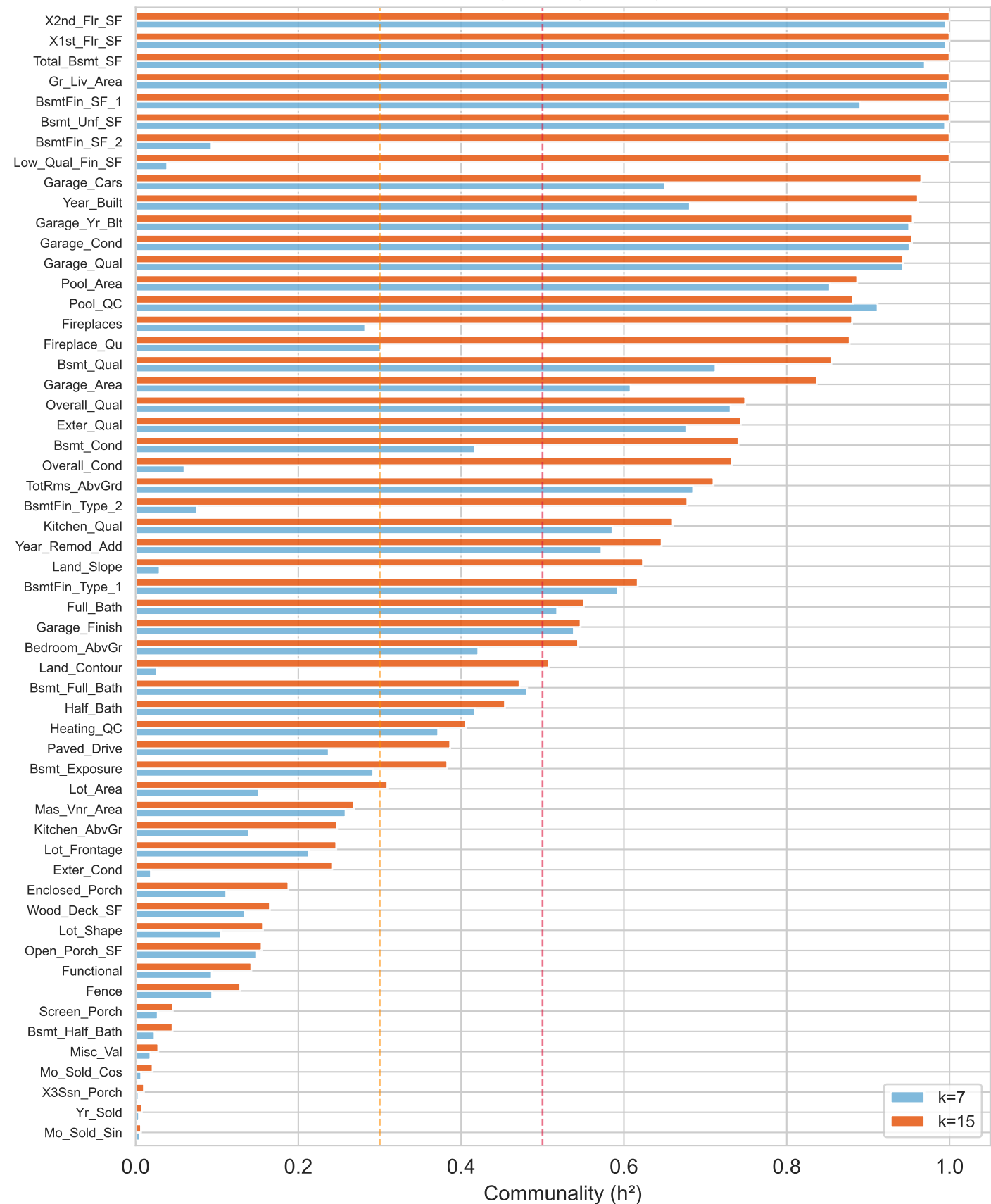
(a) Commuality: k=7 vs k=15 \Sigma h^2 gain: 8.5 (+15.1 pp)
