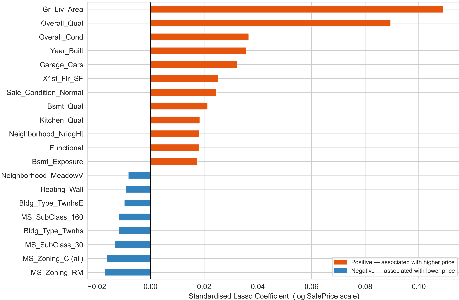
Figure 8 — Lasso Regression: Largest Coefficients \alpha = 0.00271 | 107 active features of 224
