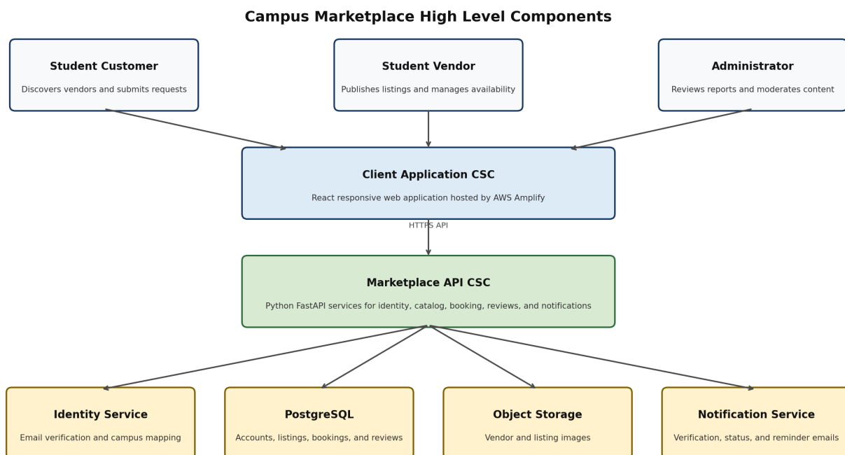
Figure 2 Campus Marketplace high level system components
