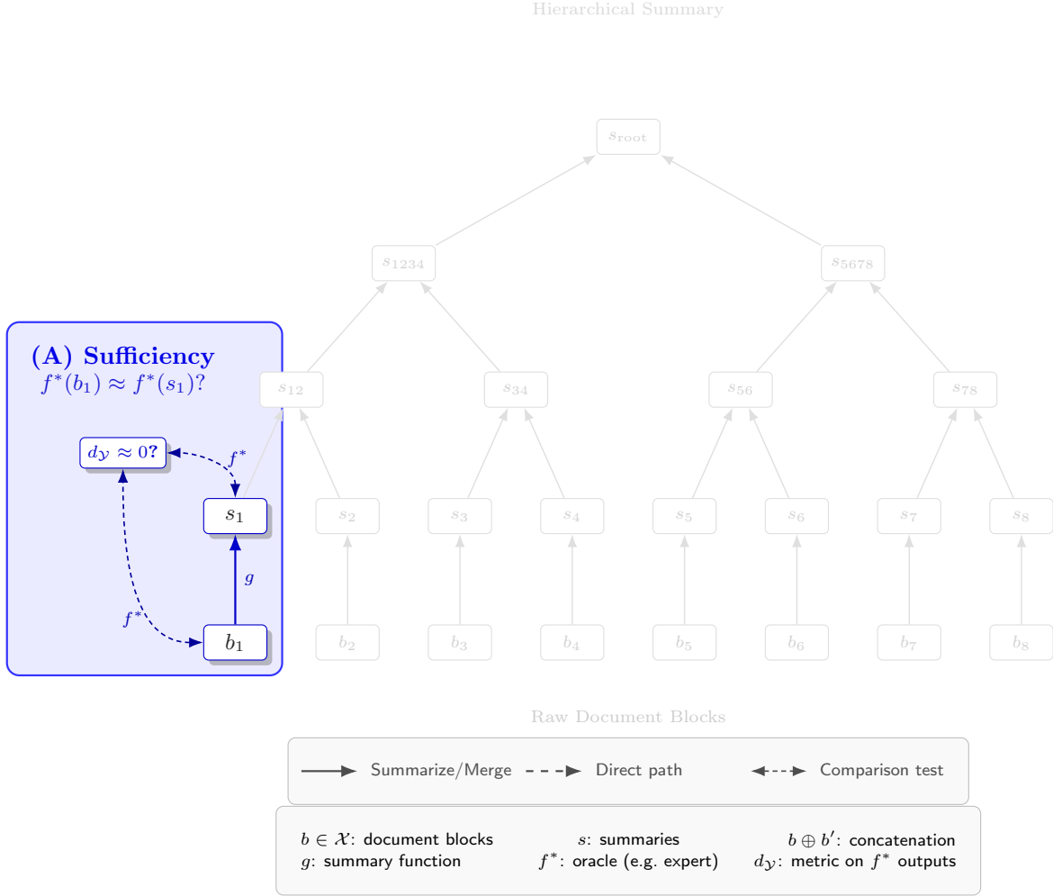
Figure 2: (A) Sufficiency: Does the summary preserve task-relevant information?
