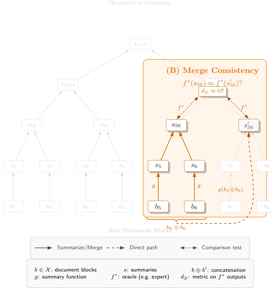
Figure 3: (B) Merge Consistency: Is the merged summary equivalent to direct summarization?
