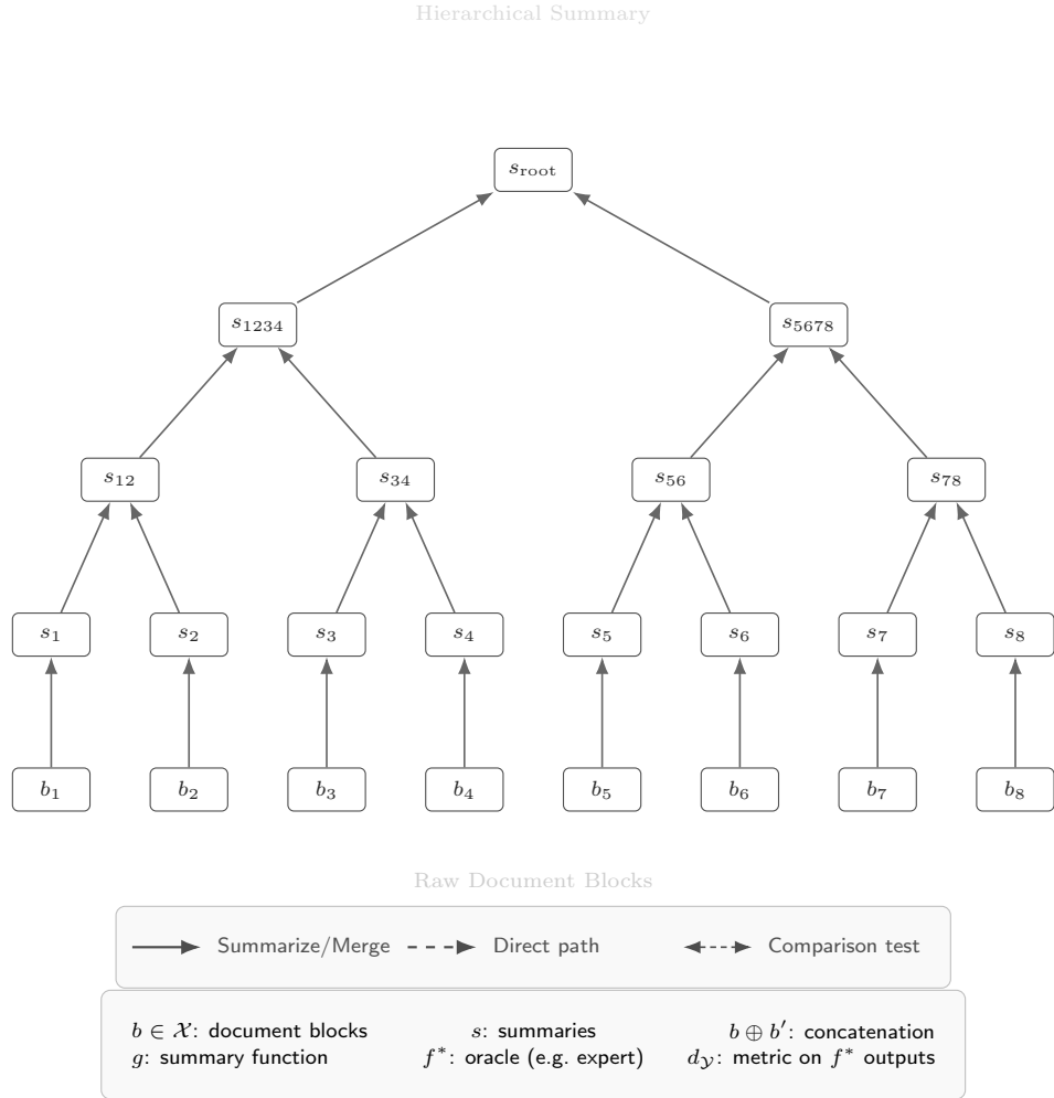
Figure 1: Base: Hierarchical Summarization Tree
