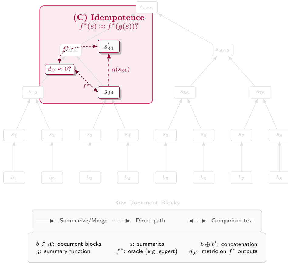
Figure 4: (C) Idempotence: Is re-summarizing a summary stable?
