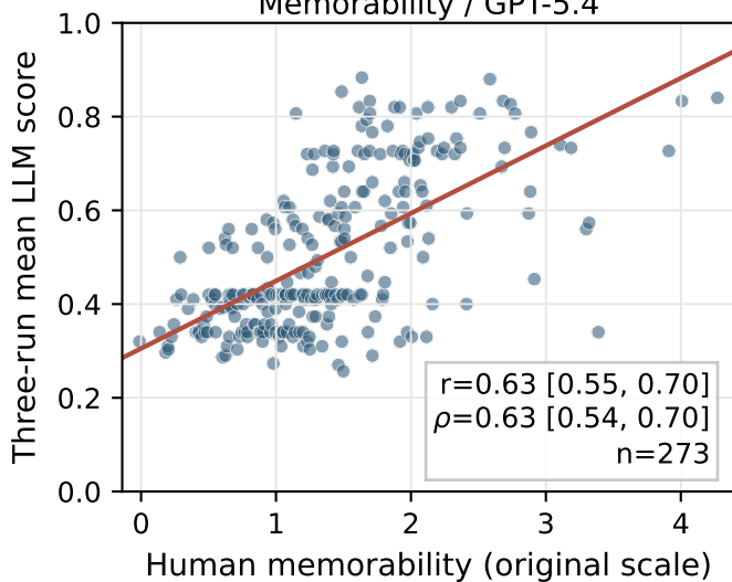
Memorability / GPT-5.4
