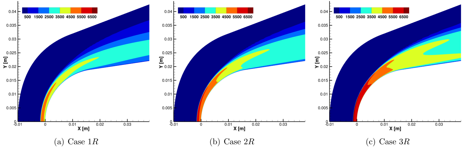
Figure 5.15: Contour vibrational temperature for nonequilibrium cases from tab. 5.7
