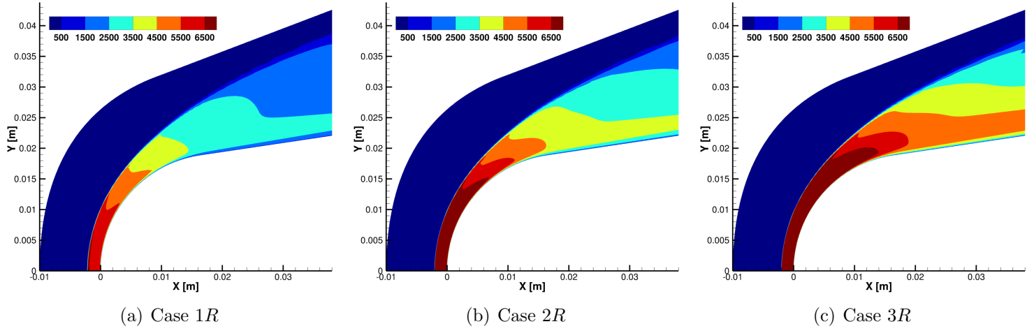
Figure 5.12: Contour translational temperature for frozen cases from tab. 5.7
