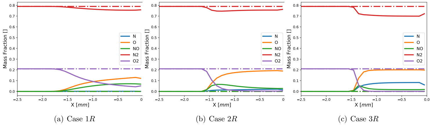
Figure 5.18: Stagnation mass fractions: solid lines represent the nonequilibrium cases, while dashed lines represent the frozen cases
