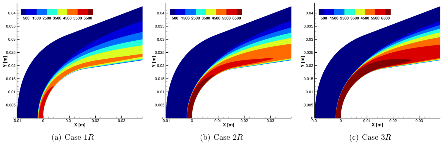
Figure 5.14: Contour vibrational temperature for frozen cases from tab. 5.7
