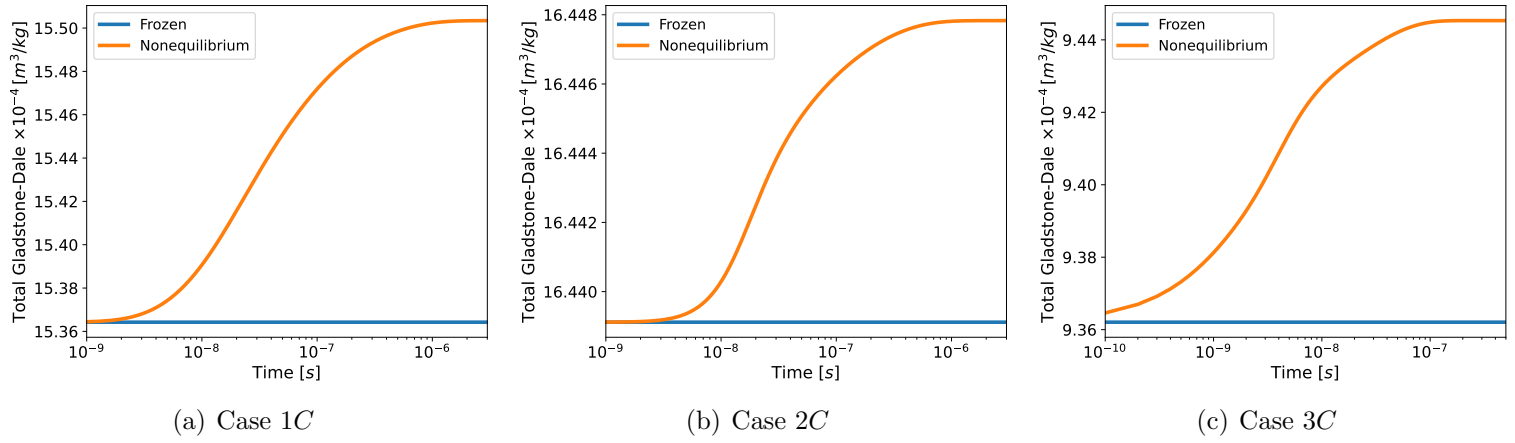
Figure 5.4: Total Gladstone-Dale results for cases in tab. 5.3
