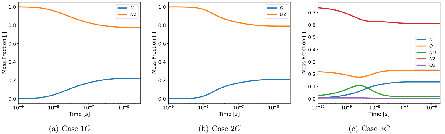
Figure 5.2: Mass fraction results for cases in tab. 5.3
