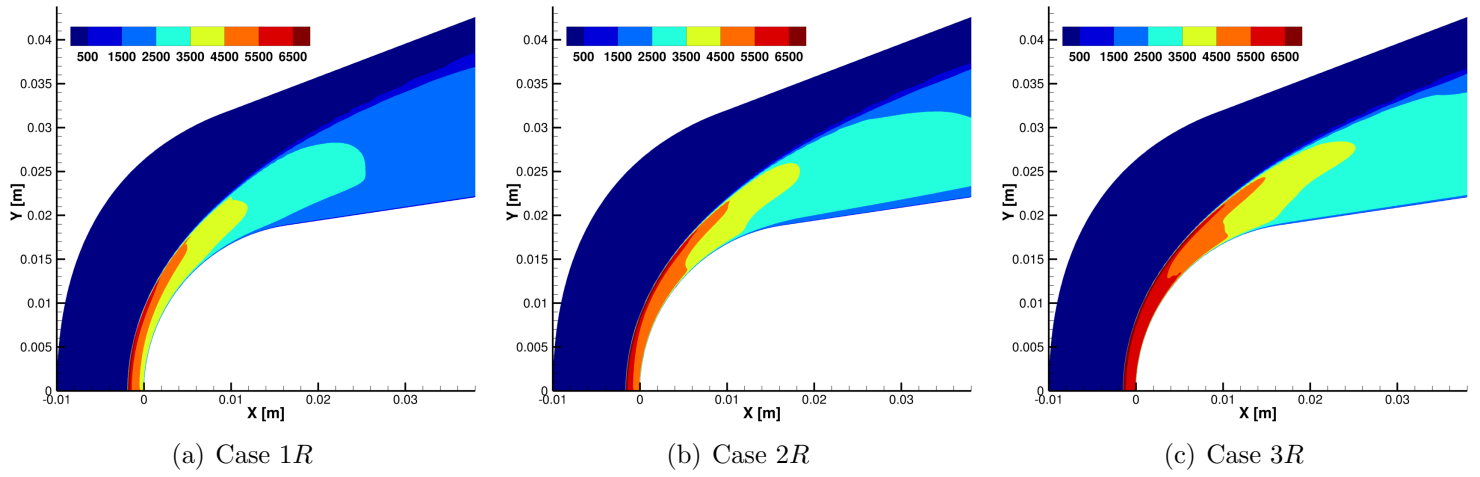
Figure 5.13: Contour translational temperature for nonequilibrium cases from tab. 5.7
