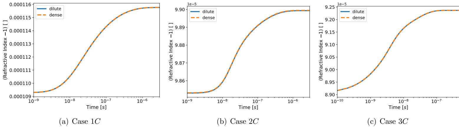
Figure 5.5: Index of Refraction results for cases in tab. 5.3
