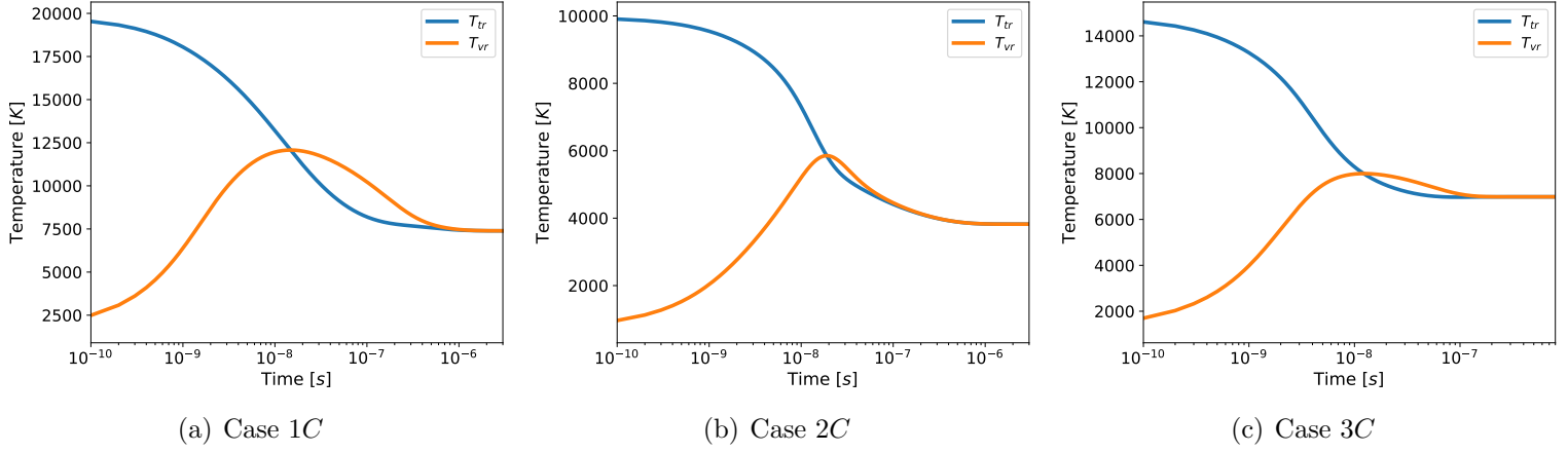
Figure 5.1: Temperature results for cases in tab. 5.3
