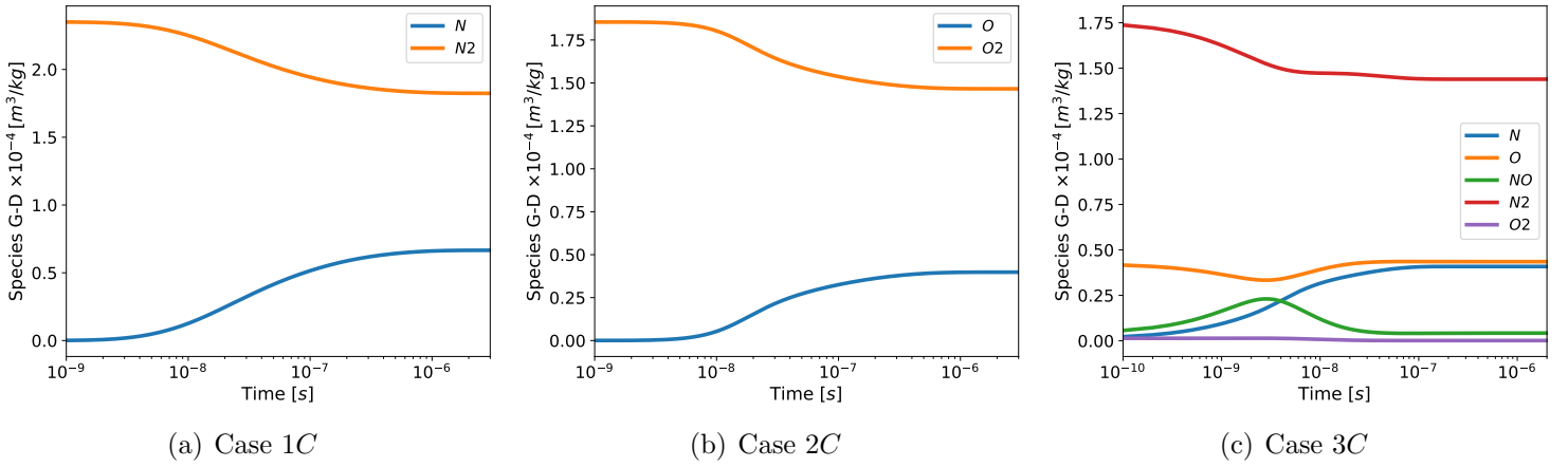
Figure 5.3: Species G-D results for cases in tab. 5.3
