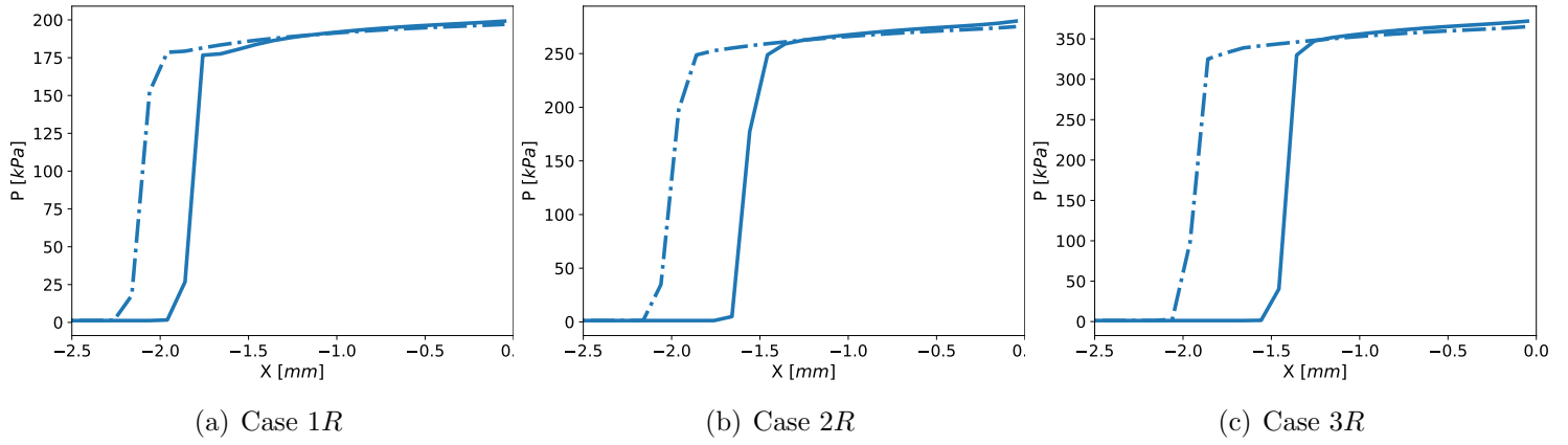
Figure 5.17: Stagnation pressures: solid lines represent the nonequilibrium cases, while dashed lines represent the frozen cases
