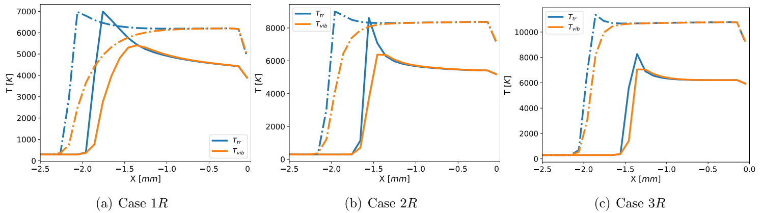
Figure 5.16: Stagnation temperatures: solid lines represent the nonequilibrium cases, while dashed lines represent the frozen cases
