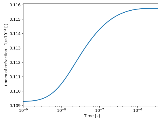
Figure 5.5: Index of Refraction for case 1H
