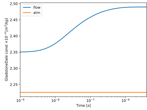
Figure 5.4: Gladstone-Dale constant for case 1H
