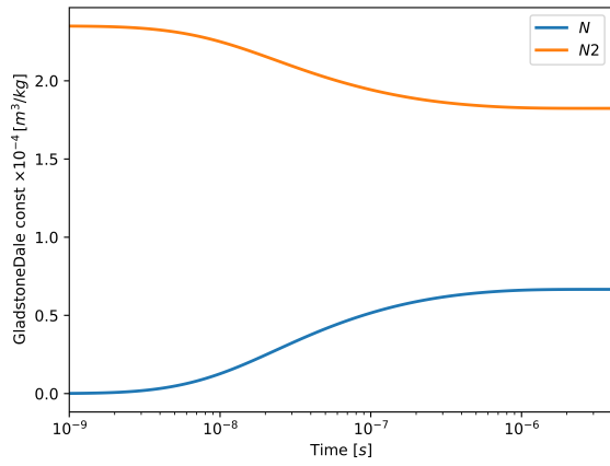
Figure 5.3: Specific Gladstone-Dale constant for case 1H
