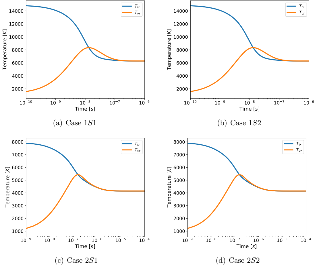
Figure 5.6: Temperature results for cases in tab. 5.5
