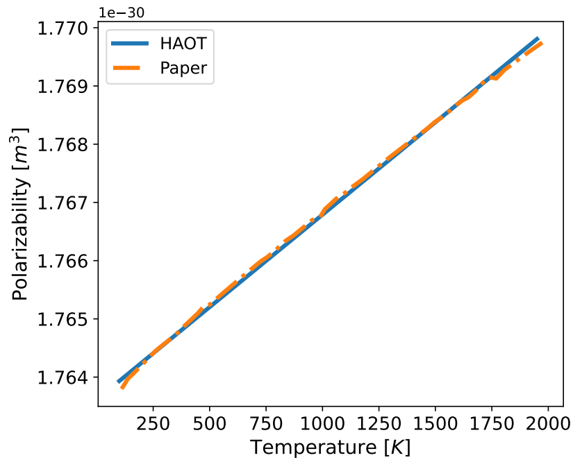
Figure 4.3: Polarizability of N_2 for a wavelength of 633 [nm]
