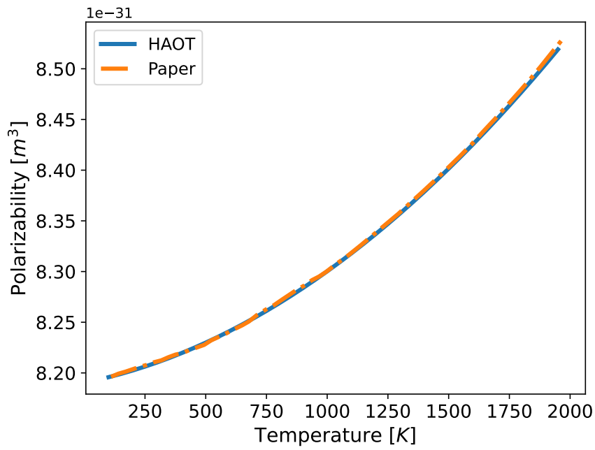
Figure 4.5: Polarizability of H_2 for a wavelength of 633 [nm]
