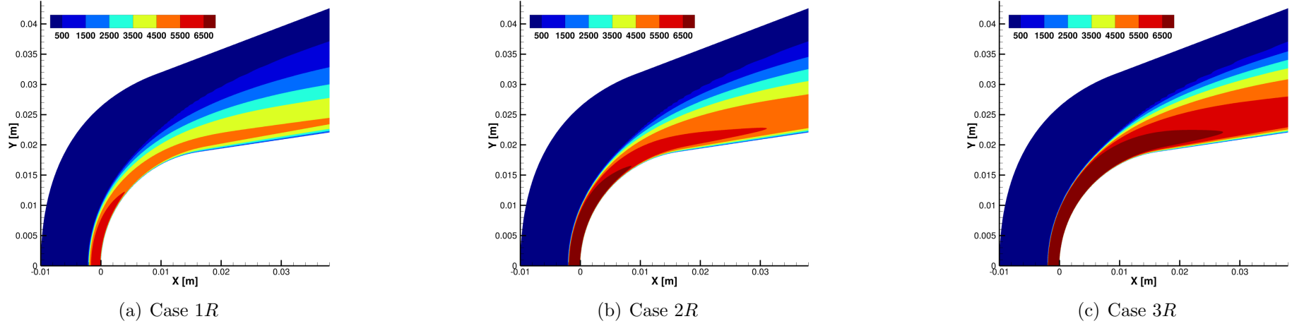
Figure 5.14: Contour vibrational temperature for frozen cases from tab. 5.7
