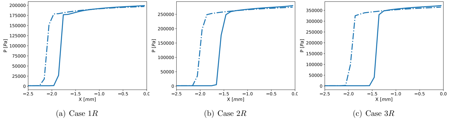
Figure 5.17: Stagnation pressures: solid lines represent the nonequilibrium cases, while dashed lines represent the frozen cases
