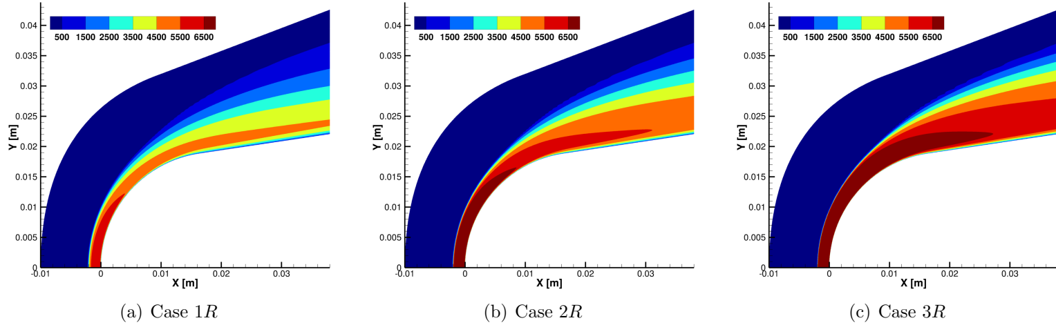
Figure 5.14: Contour vibrational temperature for frozen cases from tab. 5.7
