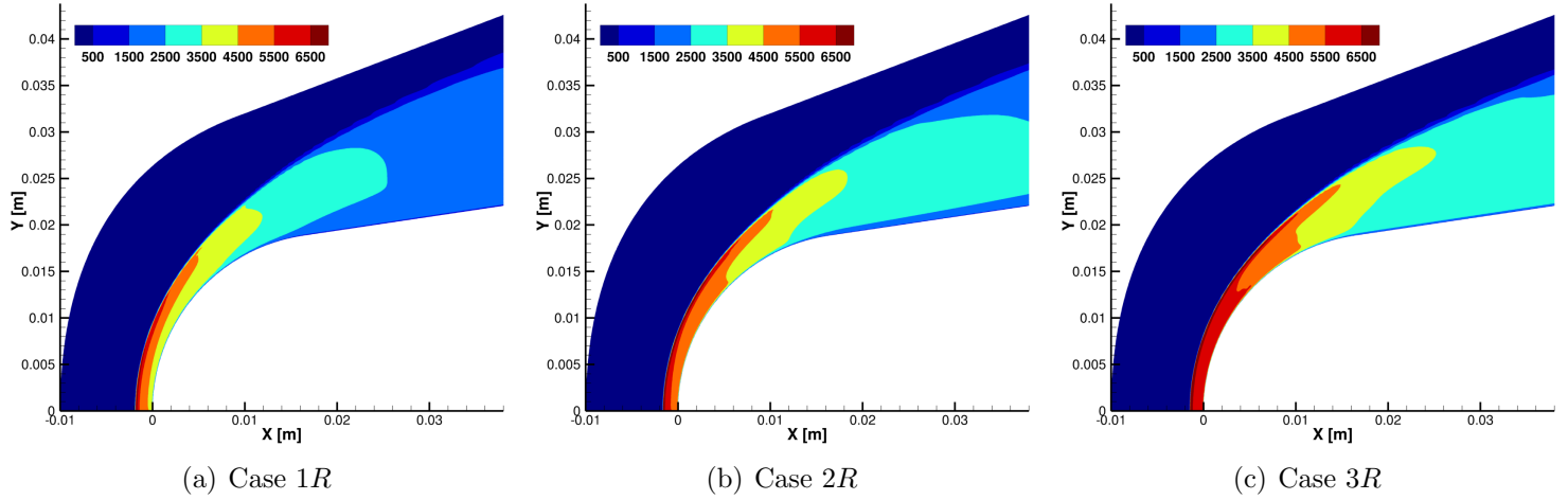
Figure 5.14: Contour translational temperature for nonequilibrium cases from tab. 5.7
