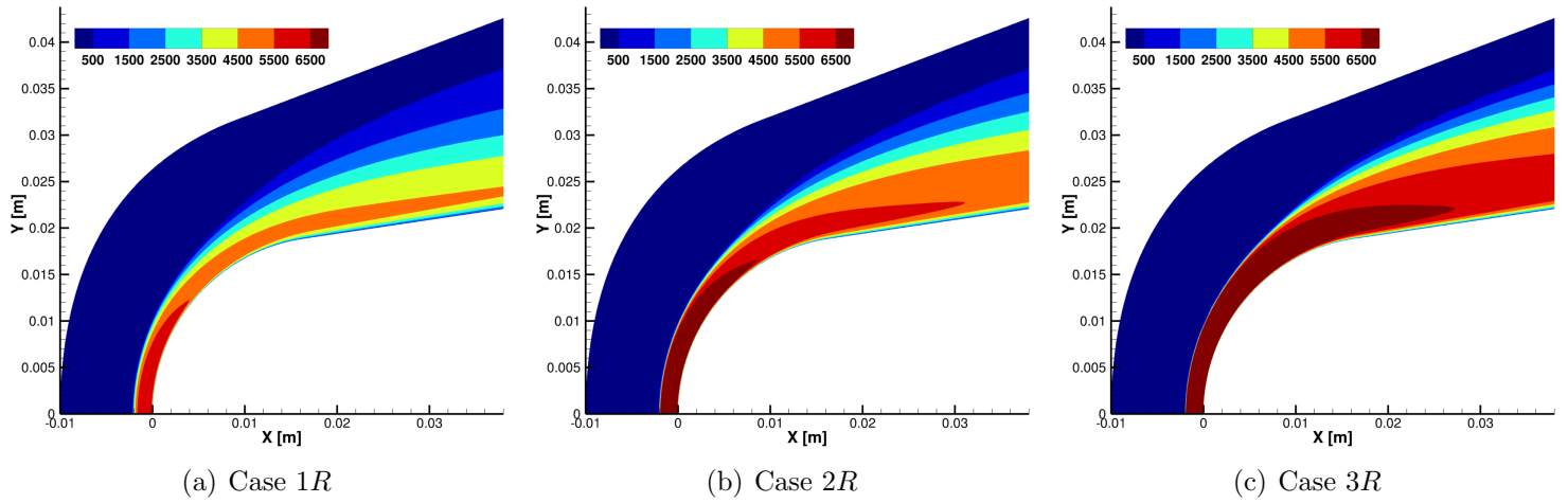
Figure 5.13: Contour vibrational temperature for frozen cases from tab. 5.7
