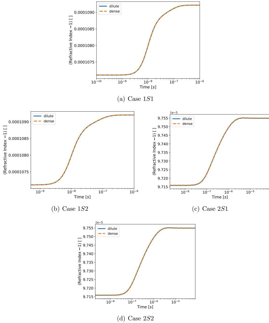
Figure 5.10: Index of Refraction results for cases in tab. 5.5
