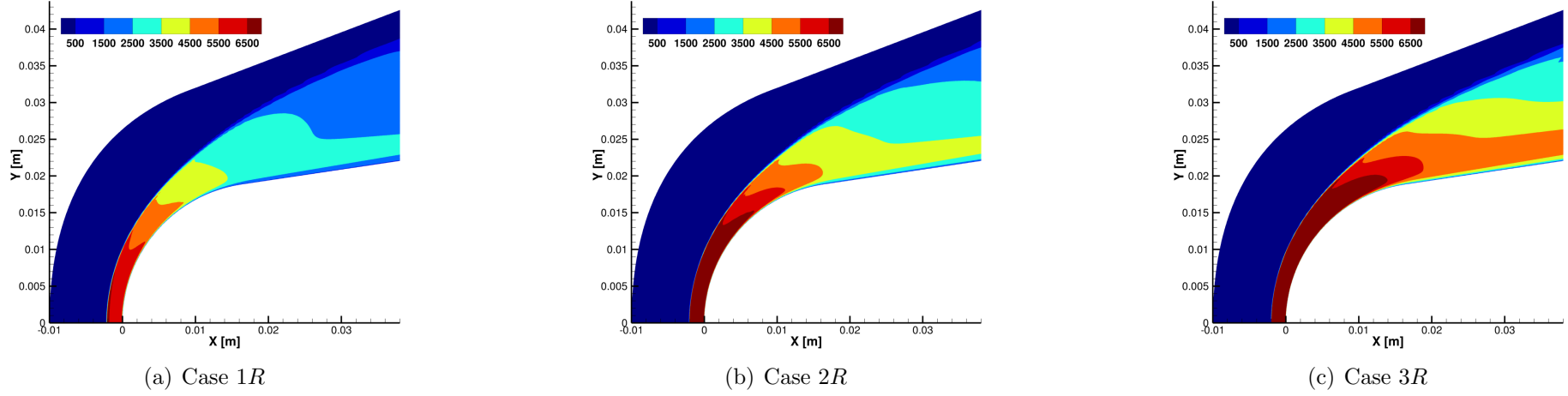
Figure 5.12: Contour translational temperature for frozen cases from tab. 5.7
