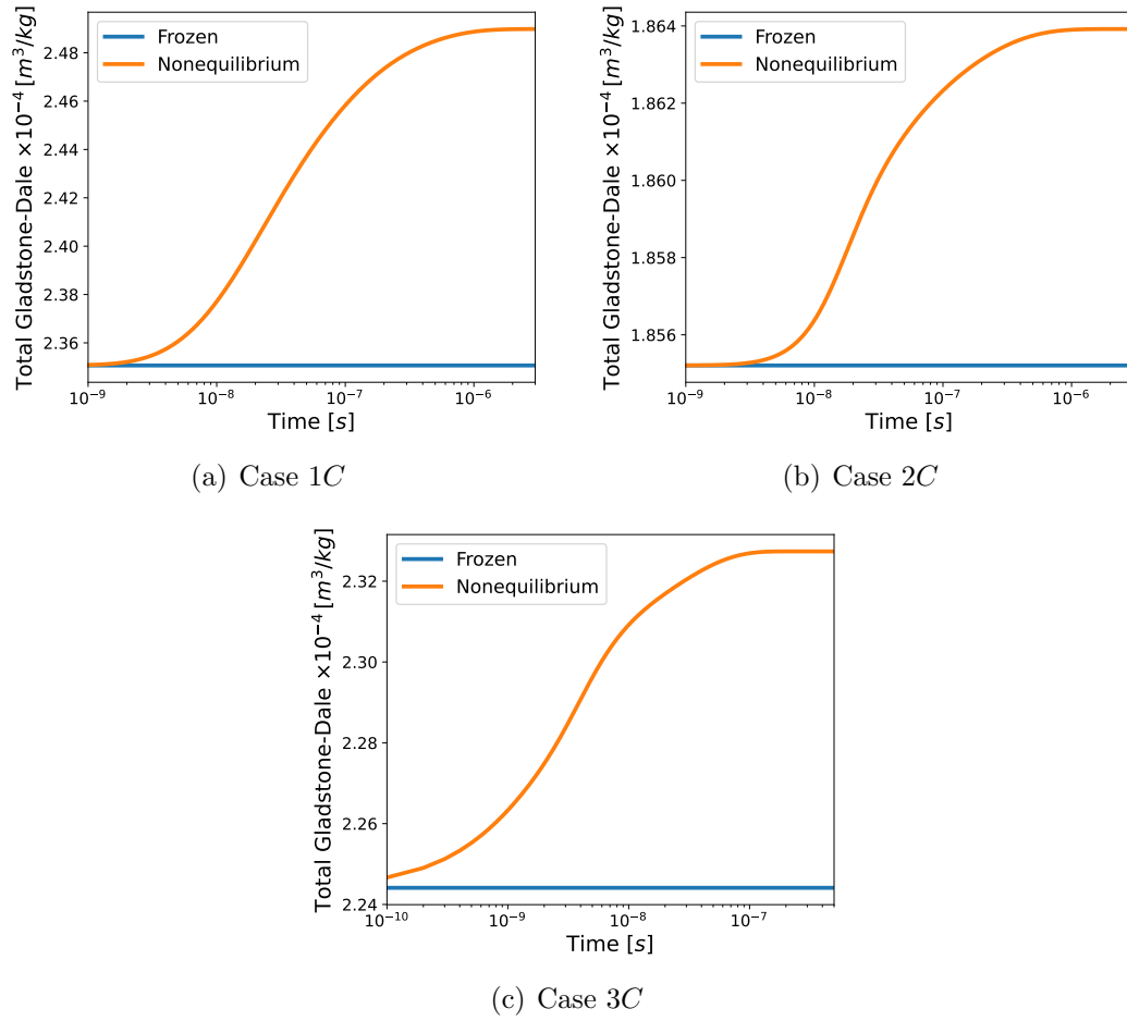
Figure 5.4: Total Gladstone-Dale results for cases in tab. 5.3
