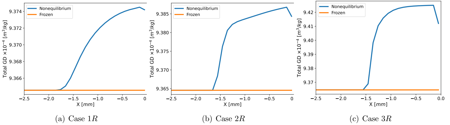
Figure 5.20: Stagnation total G-D
