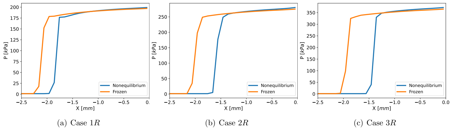
Figure 5.17: Stagnation pressures
