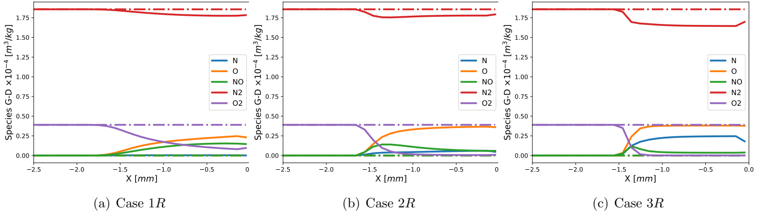
Figure 5.19: Stagnation species G-D: solid lines represent the nonequilibrium cases, while dashed lines represent the frozen cases
