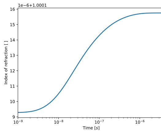
Figure 5.5: Index of Refraction for case 1H
