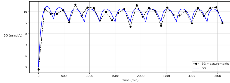
Figure 2.1: Fitting the insulin sensitivity S_I hourly using the integral-based parameter identification method on a patient model * .
