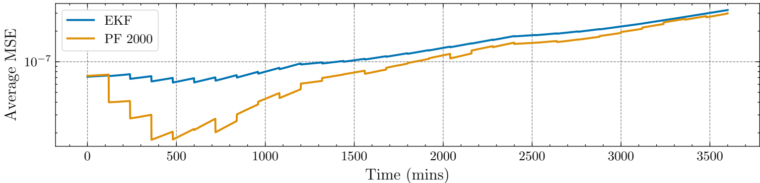
Time-varying S_I
