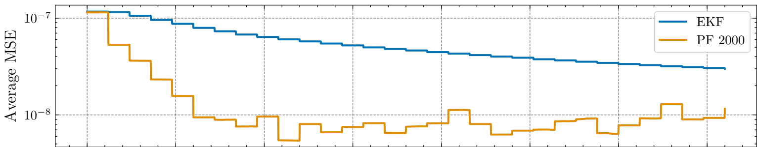
Time-varying S_I
